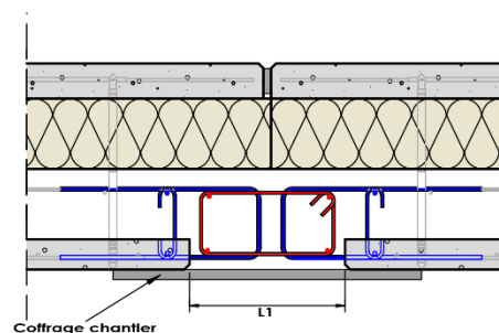
Figure 36 : Joint vertical encastré – Type Ev2
