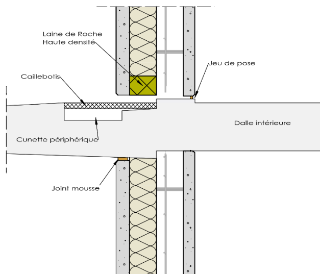
Figure 62 : Liaison (i)Premur A2C/balcon
