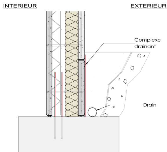
Figure 8 : Murs semi-enterrés
