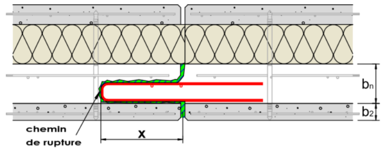
Figure 87 : plan de rupture 2
