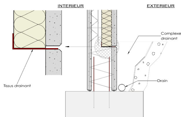
Figure 8 : Murs semi-enterrés
